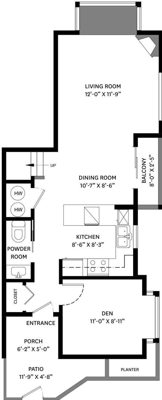
MAIN FLOOR PLAN Ceiling Height: 8'-0"
